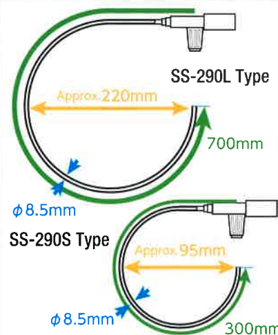
SS-290 Series Sensor Part
